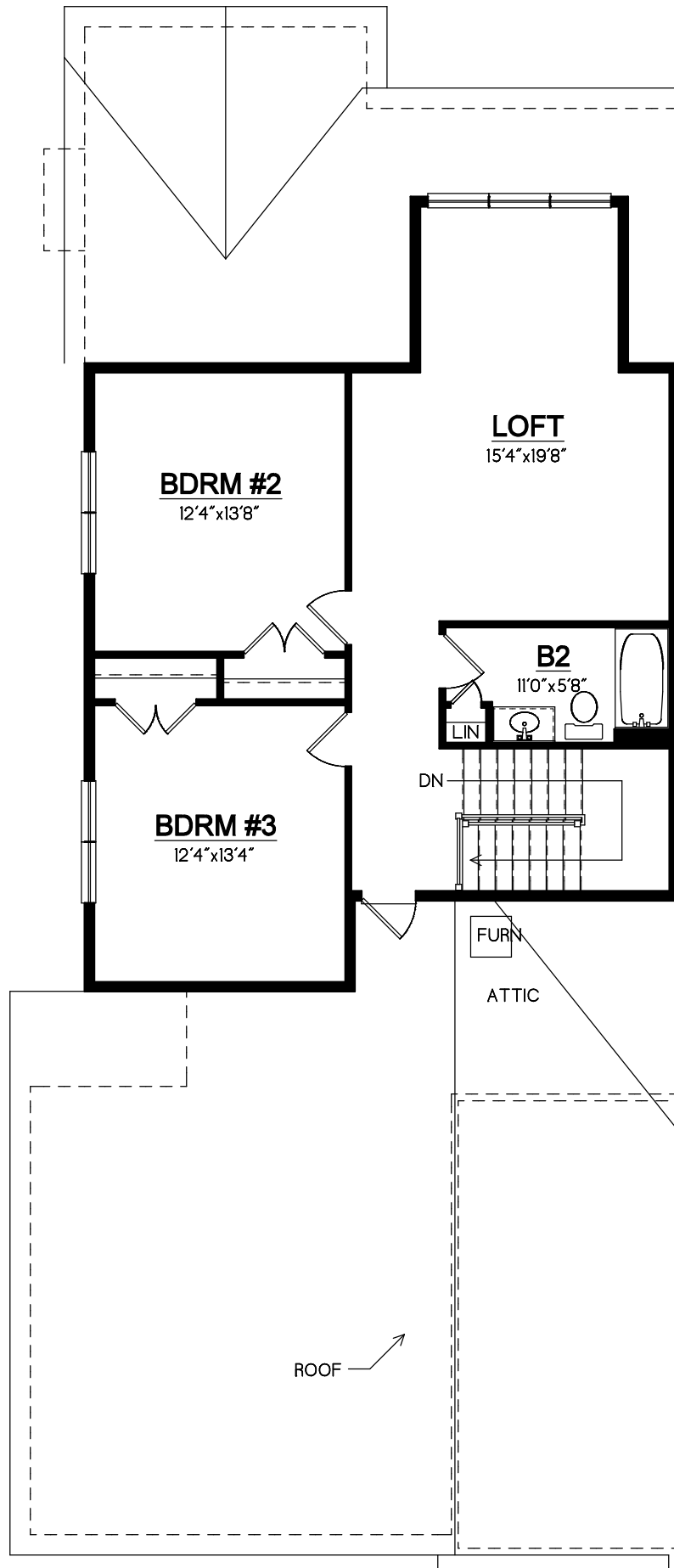
2nd Floor Scale: 1/8"=1'-0"
