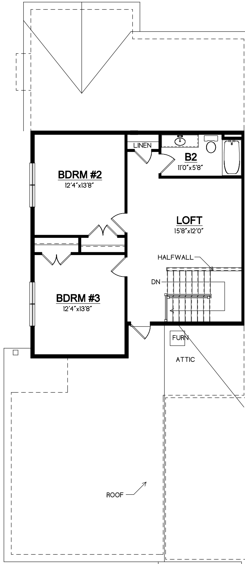
2nd Floor Scale: 1/8"=1'-0"
